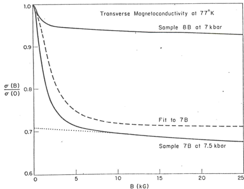
FIG. 4. Transverse magnetoconductivity as a function of magnetic field for samples 7B and 8B at 77^\circ\text{K} . The steady decrease in the conductivity at higher fields is believed to be due to geometric effects. (The sample width is approximately one-half the voltage-contact spacing, and about one-fourth of the sample length.) The asymptotic value of \sigma(\infty)/\sigma(0) was found by extrapolating the experimental curve back to zero field (dotted straight line).
