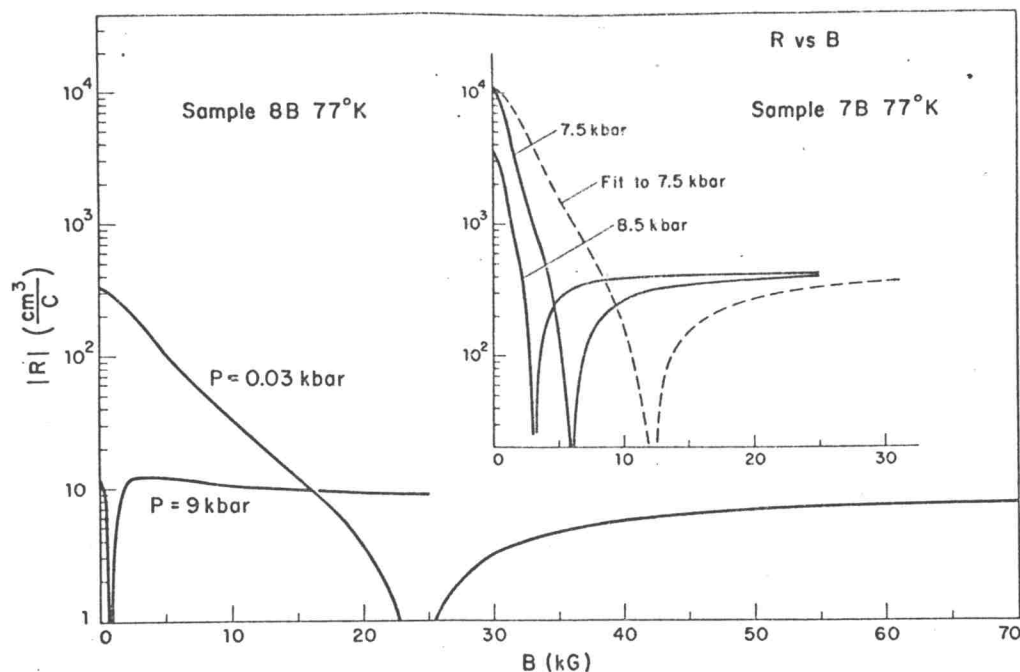
FIG. 3. Hall coefficient R as a function of magnetic field in samples 8B and 7B at 77^\circ\text{K} . R is negative for low fields and changes sign with increasing field. The fitted curve (dashed) represents the usual two-carrier expression for R with the two-carrier densities and two mobilities obtained by making the Hall coefficient and conductivity agree at B=0 and B=\infty . The lack of agreement in the crossover region is due to quantum effects (see text).
